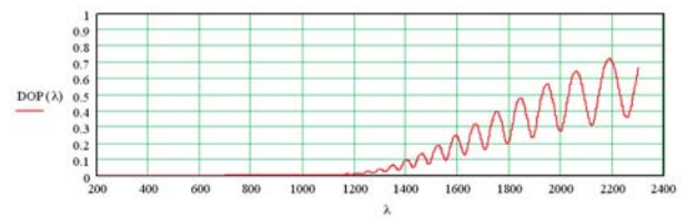
DOP Vs. input wavelength (Input beam with 100nm bandwidth, total length 6mm)
